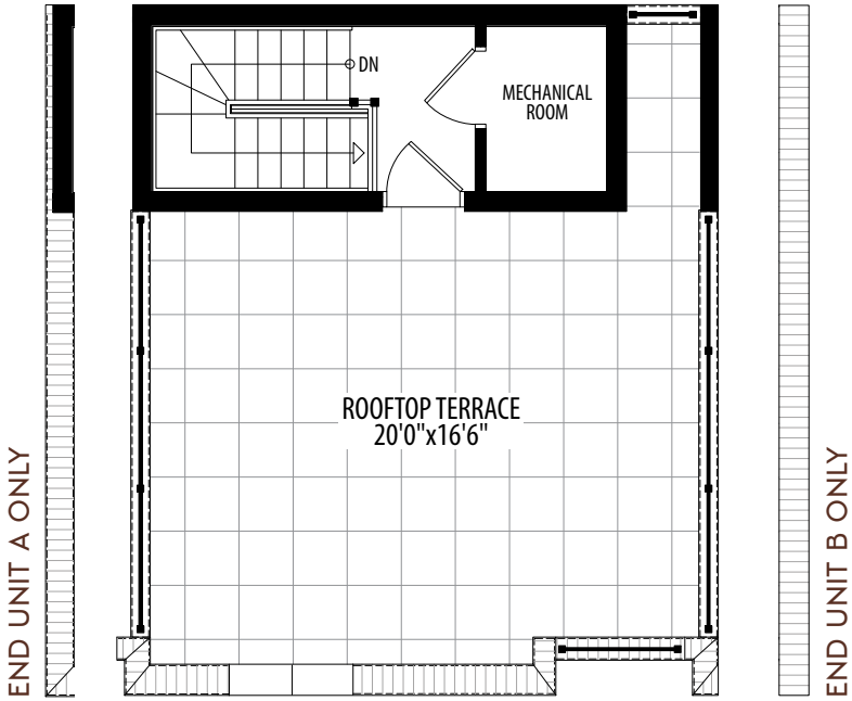
ROOF TERRACE LEVEL
